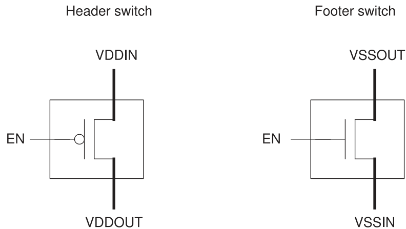
Figure 16 Power-Switch Cells
