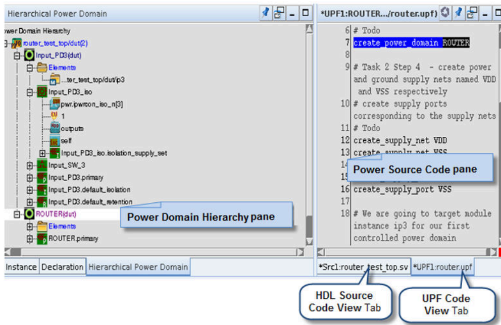
Figure 52 Power-Aware Debug
