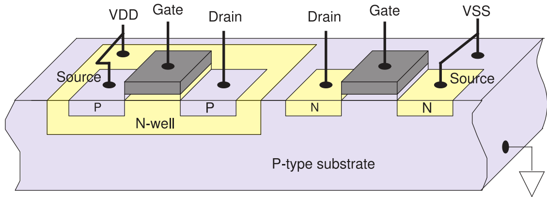
Figure 41 CMOS Technology Without Well Bias
