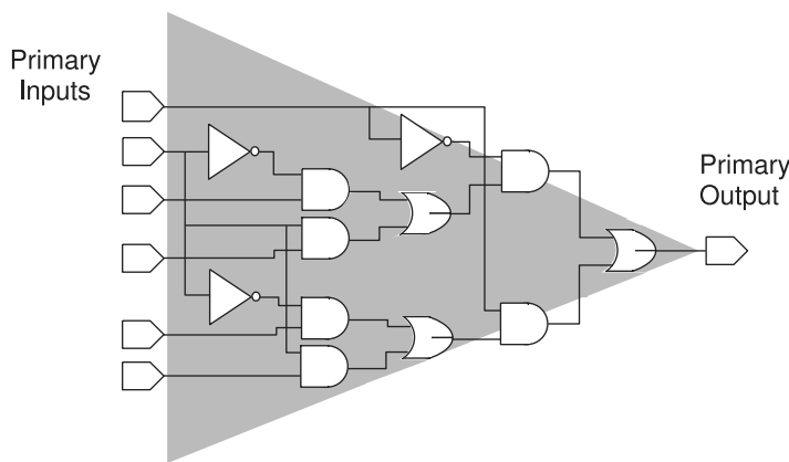
Figure 3 Logic Cone
