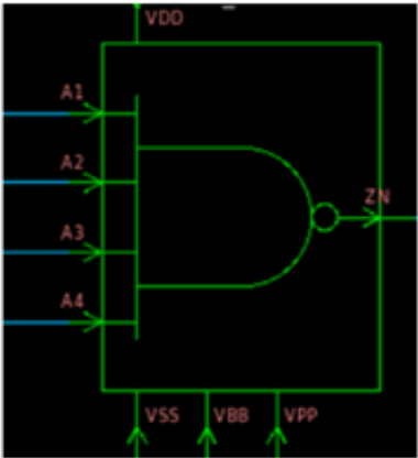
Figure 56 Power version of NAND gate
